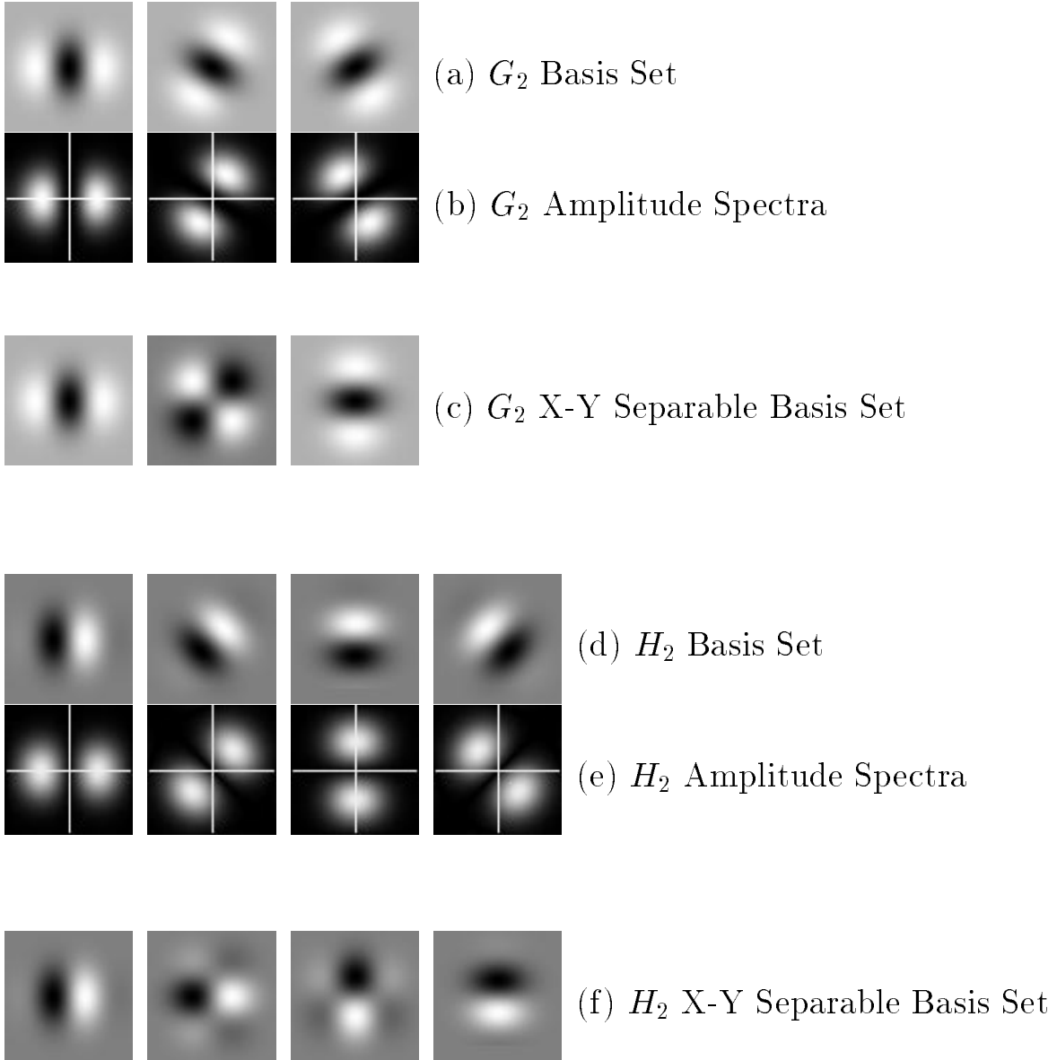
Figure 5: G_2 and H_2 quadrature pair basis filters (rows (a) and (d)). The filters in rows (a) and (d) span the space of all rotations of their respective filters. G_2 and H_2 have the same amplitude spectra (rows (b) and (e)), but 90^\circ shifted phase. Steerable G_2 and H_2 filters can measure local orientation direction and strength, and the phase at any orientation. Rows (c) and (f) show equivalent x-y separable basis functions which can also synthesize all rotations of G_2 and H_2 , respectively.
